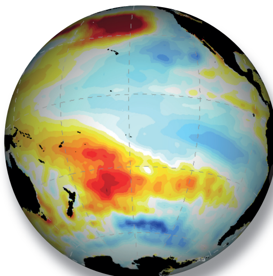
Mega-drought average
