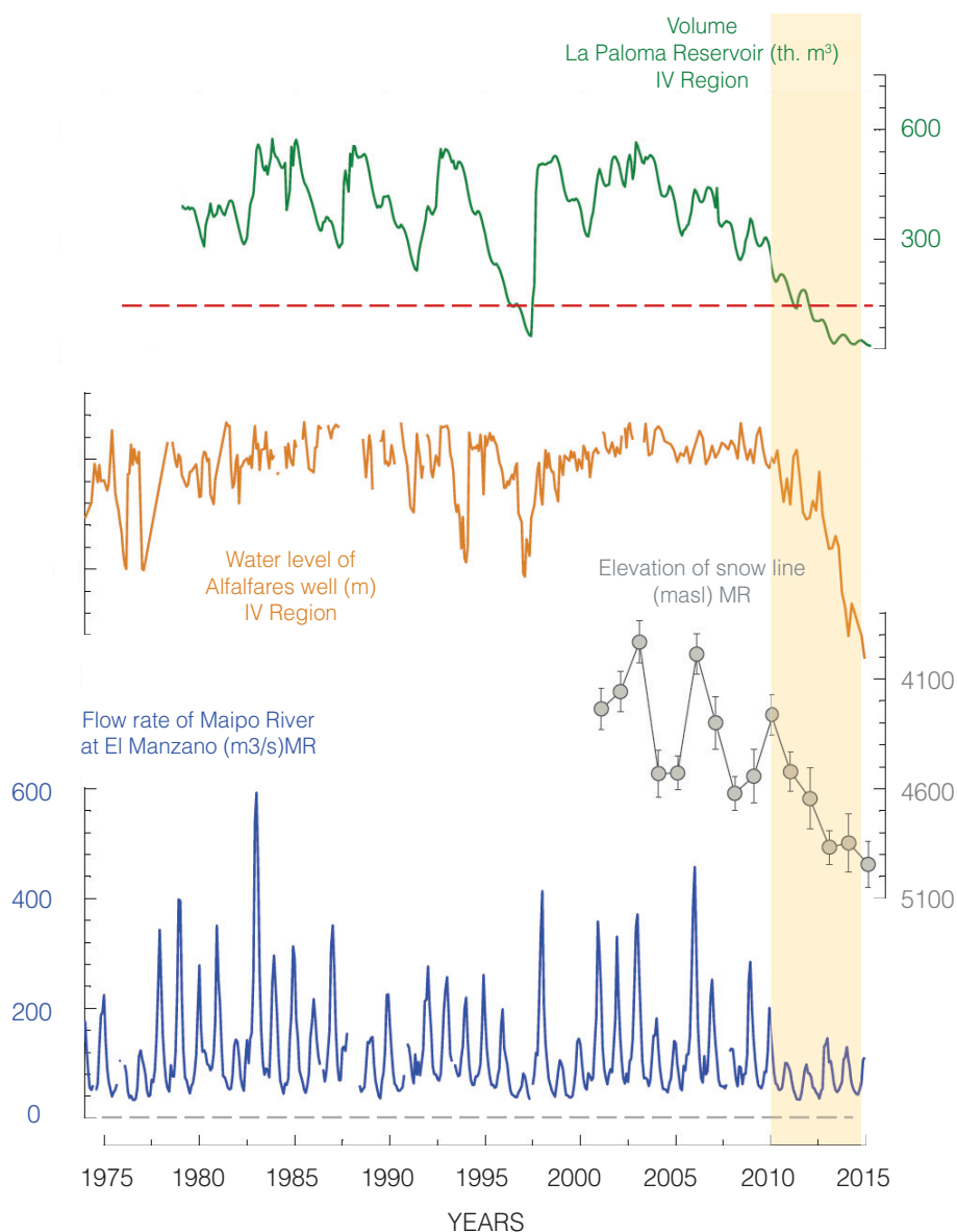
Evolution in time of water volume stored in La Paloma reservoir (green line); groundwater level in Alfalfares monitoring well (orange line); elevation of snow line during January in Andean foothills near Santiago (gray line); and flow rates at Maipo River monitoring station at El Manzano. Monthly values (except for the snow line). Data on La Paloma reservoir by kind permission of Pablo Álvarez at Universidad de La Serena. Data on Alfalfares monitoring well and on flow rates: General Water Authority. Snow line data: National Snow and Ice Data Center, USA
